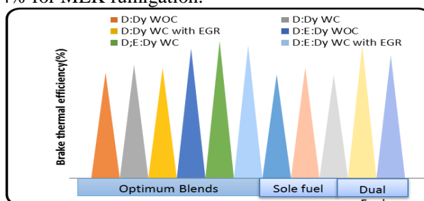
Figure.4. Comparison of brake thermal efficiency for different blends and dual fuel at peak load
