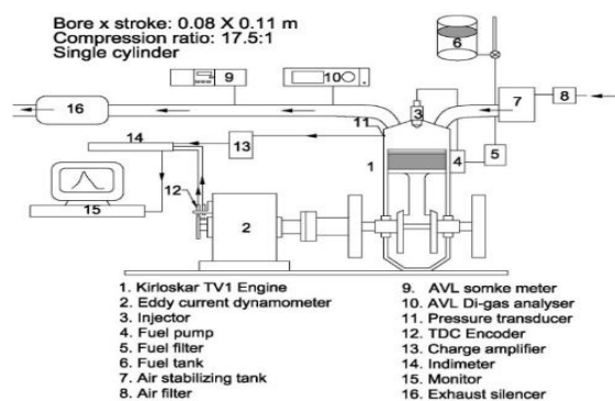
Figure.2. Experimental setup
