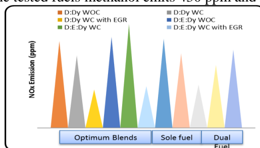
Figure.6. Comparison of NO x emissions for different blends and dual fuel at peak load
