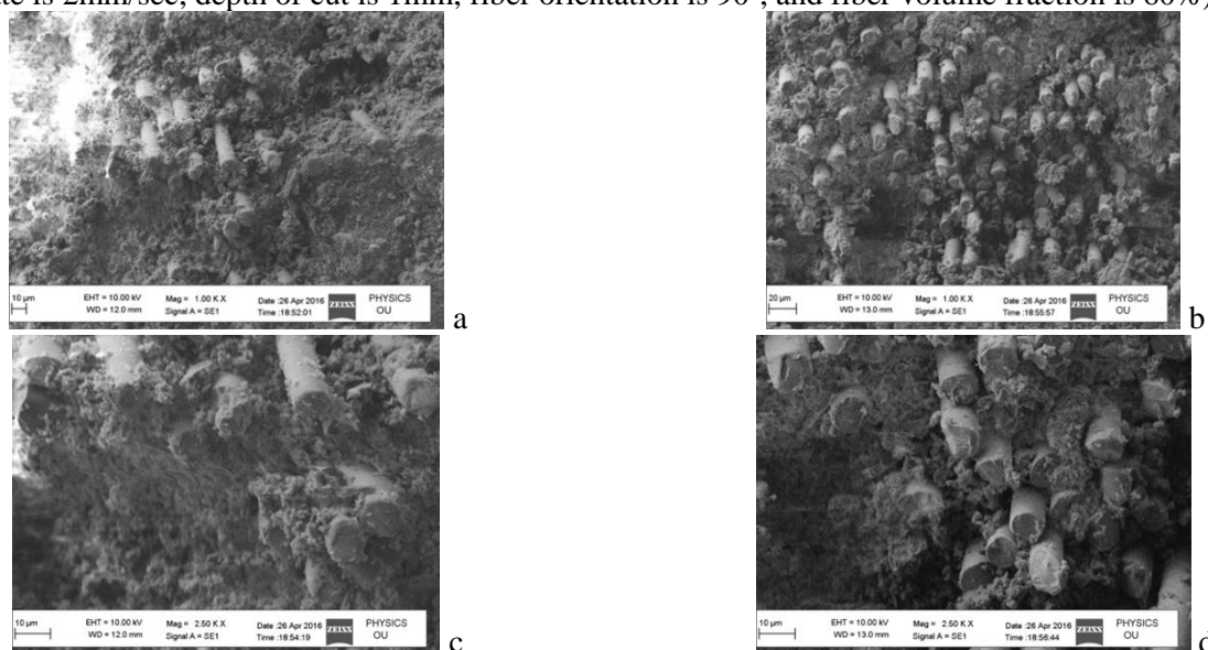
Figure.6 (a, b, c, and d). Scanning Electron Micrographs of Machined Surfaces
