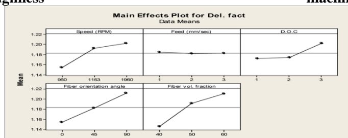
Figure.5. Illustration of factors effects on delamination factor
