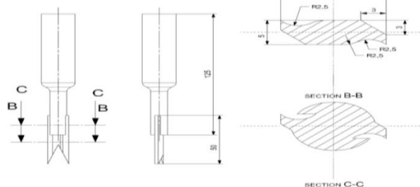
Figure. 2. Details of specially designed carbide tipped end mill tool
