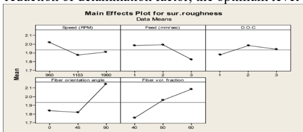
Figure.3. Illustration of factors effects on surface roughness
