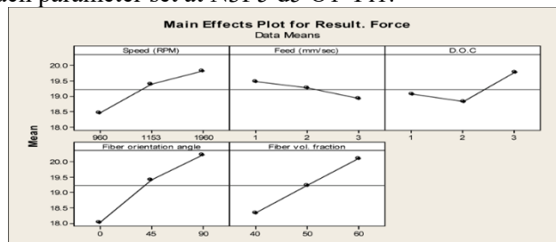
Figure.4. Illustration of factors effects on machining force
