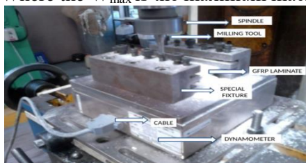
Figure.1(a). Machining of GFRP laminate plate is properly fixed in machining center by special designed fixture
