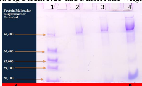
Figure.7. SDS-Polyacrylamide Gel Electrophoresis Pattern of (A) single band of RCP from Guinea pig serum (B) purification steps in DEAE-sepharose, Sephadex G-100, Riboflavin carrier protein (RCP) of Guinea Pig Serum
