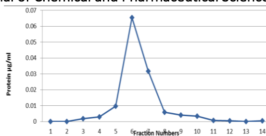
Figure.4. The partially purified Riboflavin carrier protein (RCP) was eluted from Sephadex G-100 Using Phosphate buffer pH 7.3 containing 0.5M NaCl. The protein concentration was estimated by the method of Lowry method.
