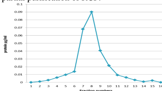
Figure.2. The partially purified RCP was eluted from DEAE-Sephadex Using Phosphate buffer pH 7.3 containing 0.5M NaCl. The protein concentration was estimated by the method of Lowry method.
