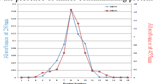
Figure.1. Guinea Pig Serum RCP elution profile on DEAE-Sephadex
