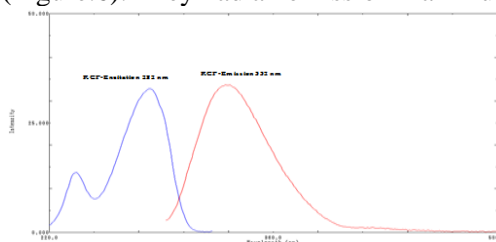
Figure.6. Fluorescence spectrum of Riboflavin Carrier protein (RCP) Excitation and emission
