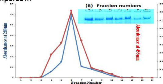
Figure.3. Guinea Pig Serum Riboflavin carrier protein elution profile on Sephadex G-100 and (B) Fraction no (4, 5, 6, 7, 8, 9, 10) SDS-Polyacrylamide Gel Electrophoresis Pattern of Riboflavin carrier protein (RCP) from Guinea Pig Serum.
