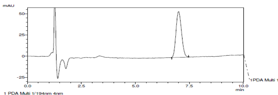
Figure.3. Representative chromatogram of 100.00 µg/mL of standard solution of Carisoprodol
