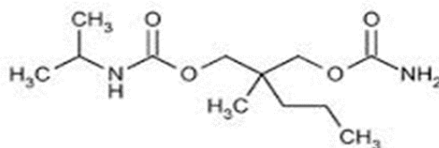
Figure.1. Chemical structure of Carisoprodol
