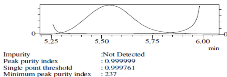
Figure.5. Chromatogram and peak purity curve for Carisoprodol in 1N NaOH at room temperature (8hr)
