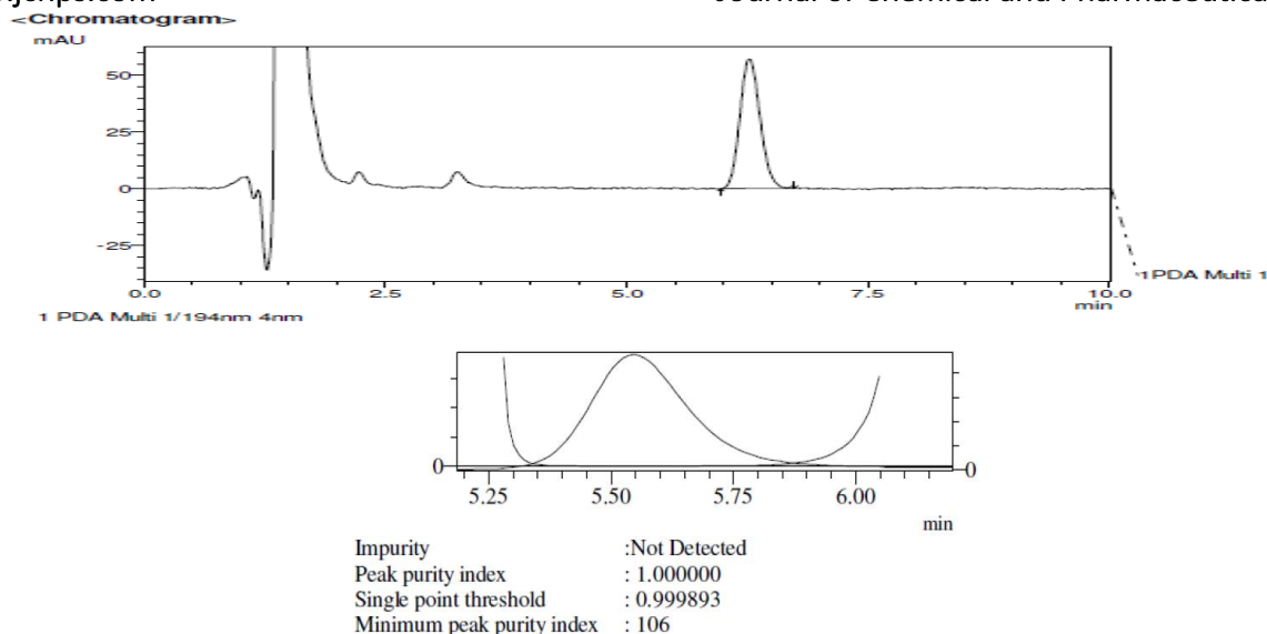
Figure.7. Chromatogram of 250.00µg/mL tablet (test) solution
