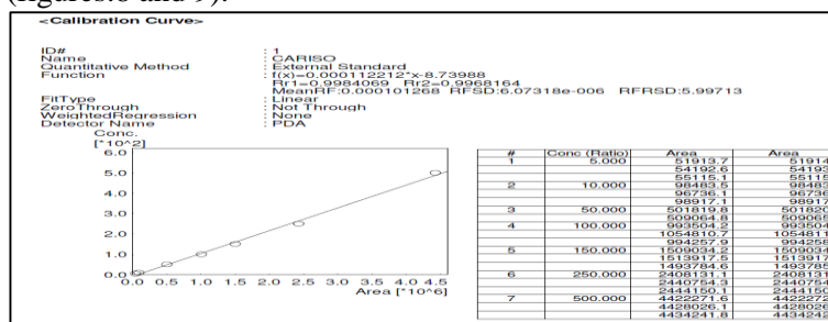
Figure.2. Calibration curve of Carisoprodol by HPLC
