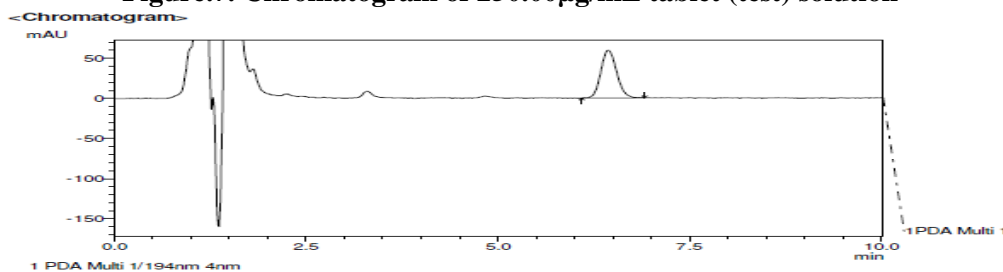
Figure.8. Representative chromatogram of marketed Carisoprodol tablets showing drug release at 60min.
