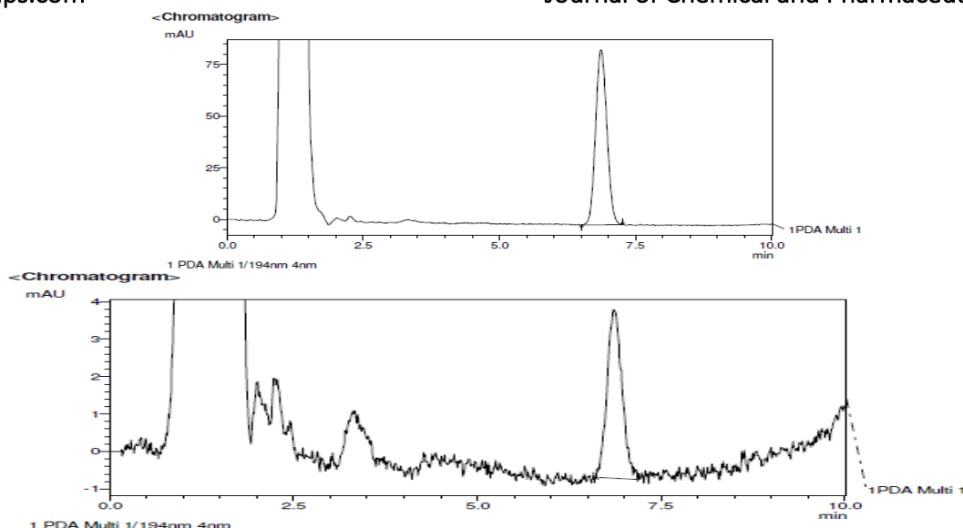
Figure.4. Chromatogram and peak purity curve for Carisoprodol in 1N HCl at room temperature (8hr)
