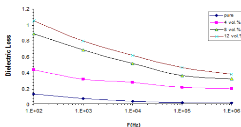
Figure.3. Variation dielectric loss for (PVA-VLO) bio composites with frequency at room temperature
