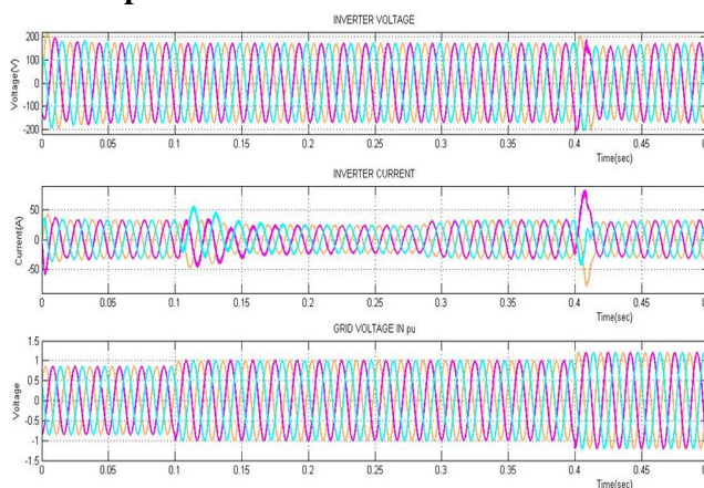
Figure.6. Output waveform of Inverter output voltage and current
