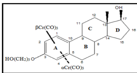
Figure.1. Optimized structures of estradiol isomer complexes with \text{Cr}(\text{CO})_3
