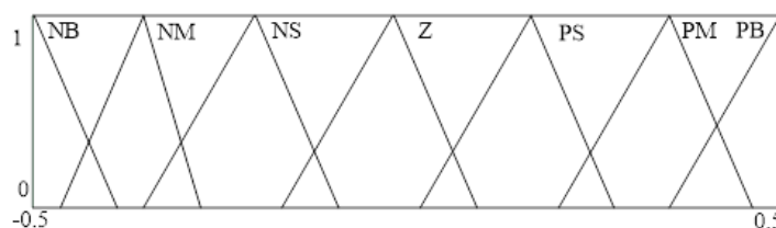
Figure.4. Membership functions of inputs and outputs for proposed controller
