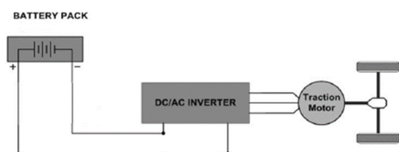
Figure.1. Conventional Topology
