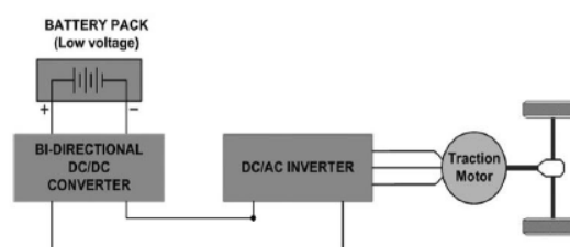
Figure.2. The Proposed Topology
