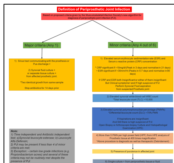
Figure 1: Flowchart of major and minor criteria of per prosthetic joint infection
