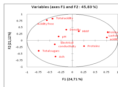
Figure.1. Principal Component Analysis (PCA)
