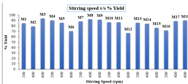
Fig. 11: Effect of Stirring speed on % Yield
