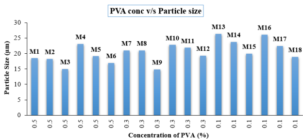
Fig. 9: Effect of PVA concentration on Particle size
