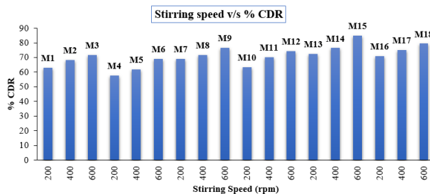
Fig. 14: Effect of Stirring speed on % CDR
