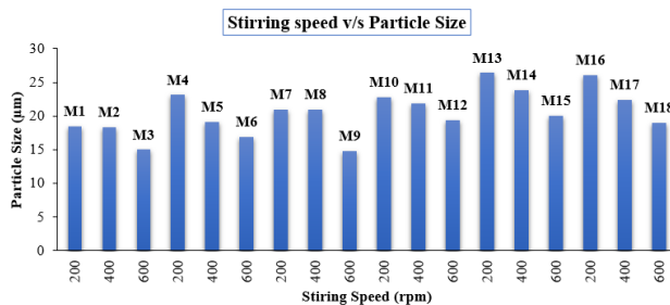
Fig. 13: Effect of Stirring speed on particle size
