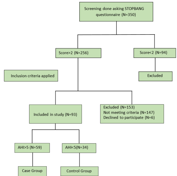
Figure 1: Flow diagram of study population selection
