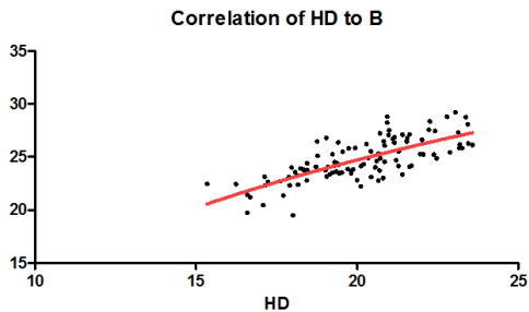
Figure 7: Scatter plot showing the correlation between the Radial Head (HD) to Distal Metaphysial Breadth (B) (Correlation: HD-mm versus B-mm, Pearson correlation= 0.7367, P-value < 0.0001)
