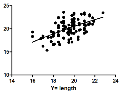
Figure 5: Scatter plot showing the correlation between the Radial Bow length(Y) to Radial head size (HD). (Correlation: Y-cm versus HD-mm, Pearson correlation= 0.5580, P-value < 0.0001)
