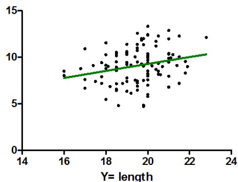
Figure 4: Scatter plot showing the correlation between the Radial bow length (Y) to Maximum bow(BW). (Correlation: Y-cm versus BW-mm, Pearson correlation= 0.2476, P-value =0.0109)
