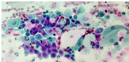
Figure 2: Pap smear and histopathological findings of a 62-year-old female, presenting with cervical growth, Pap smear showing dysplastic squamous epithelial cells, interpreted as high-grade squamous intra-epithelial lesion (HSIL). (40X; Pap stain).
