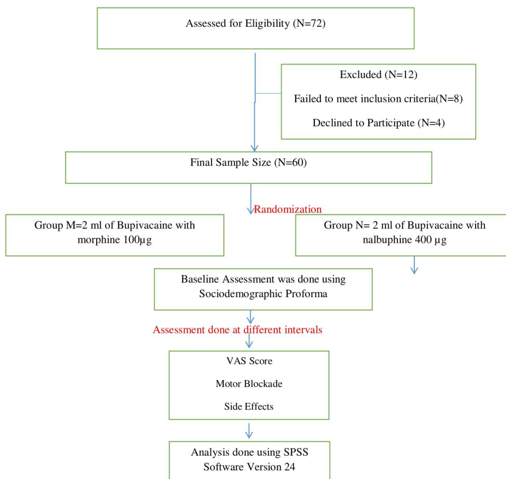
Diagram 1: Consort diagram
