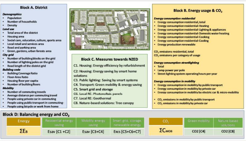
Figure 19 Building blocks of the NZED model
