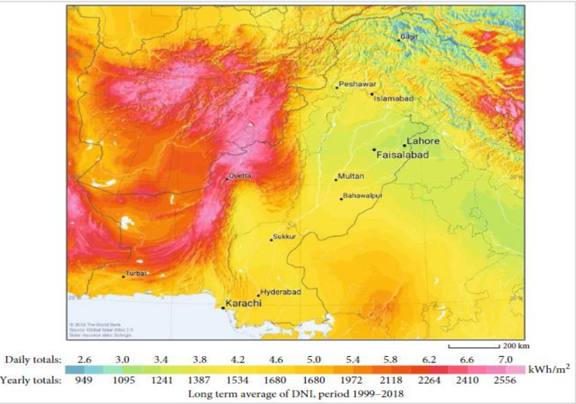
Figure 7 DNI map of Pakistan with suitable locations (Multan, Bahawalpur, Rahim Yar Khan, Hyderabad, Quetta, and Toba)
