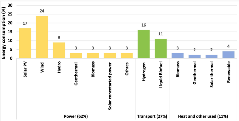
Figure 1 Analysis of renewable energy utilization in final energy consumption: REM perspective for 2050
