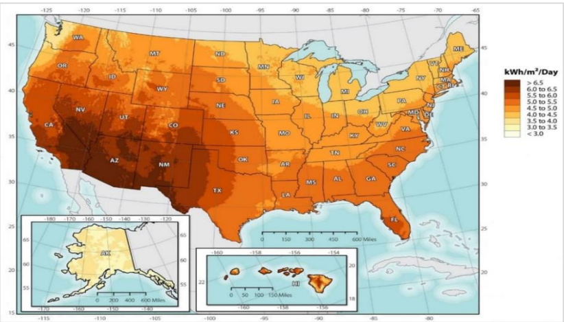
Figure 3 Solar Resources in North America
