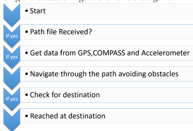
Figure 5 Navigation algorithm
