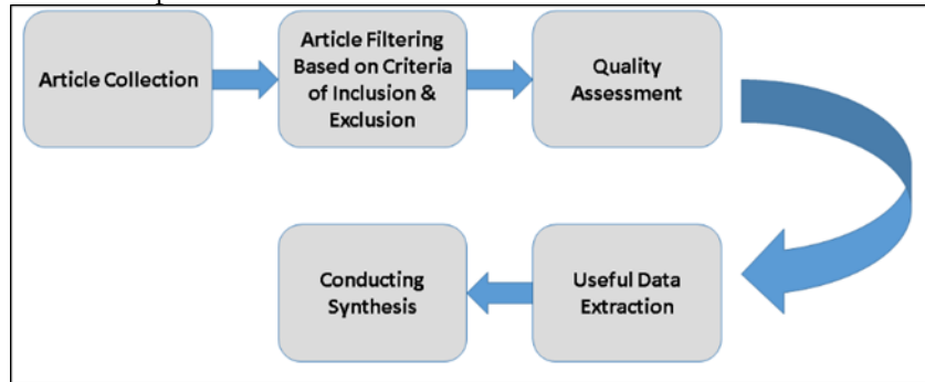
Figure 3 Methodology Flow
