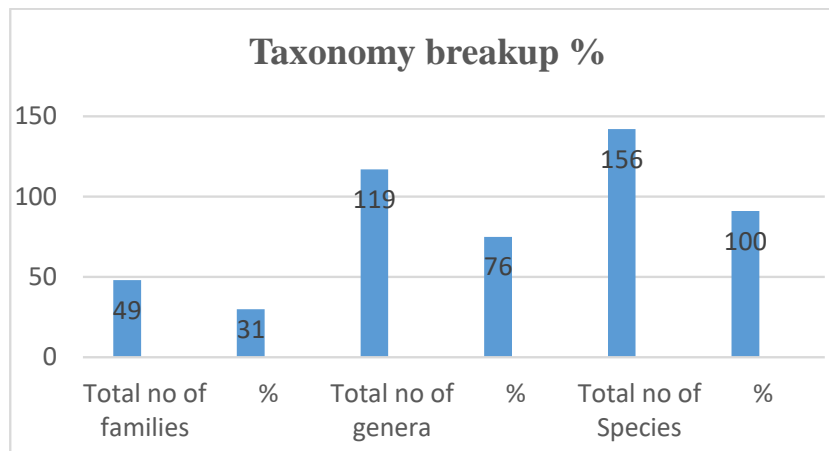
Figure 3: Taxonomy breakup with percentage.
