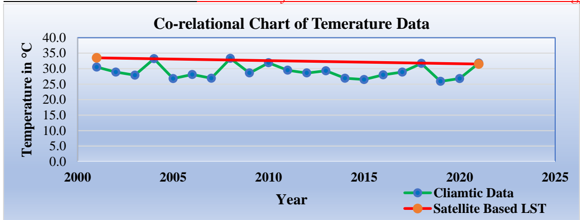
Figure 5. Co-relational chart of Temperature Data.
