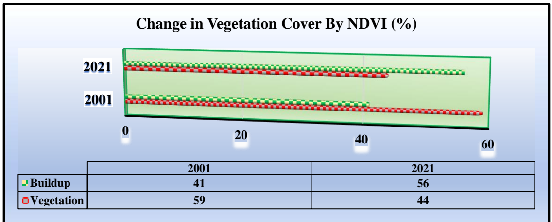
Figure 2. Normalized Difference Vegetation Index (2001 to 2021)
