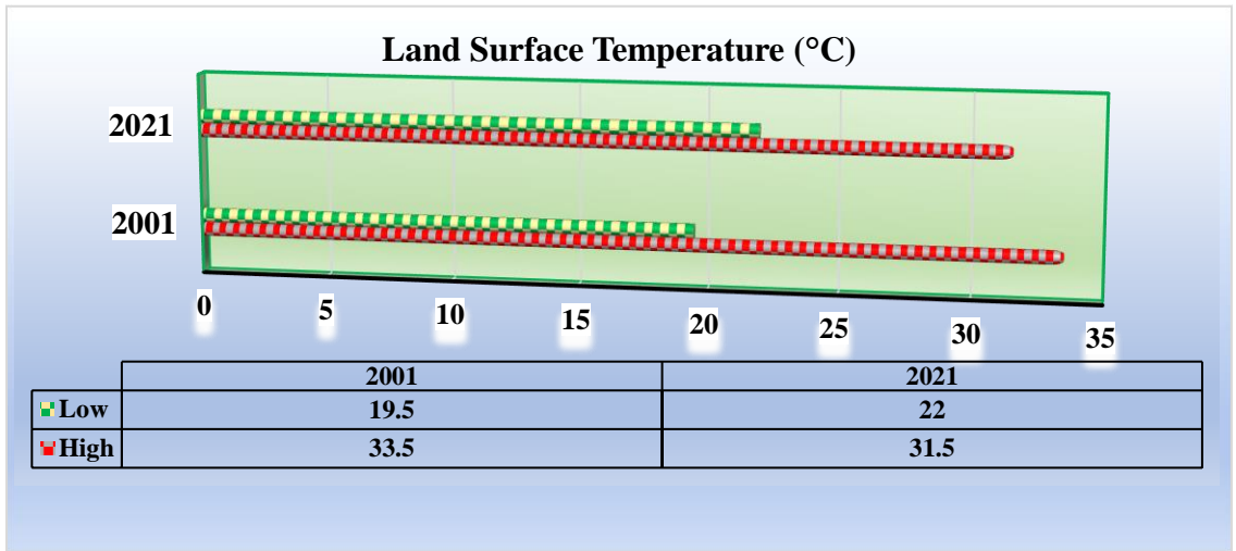
Figure 3. Land Surface Temperature (2001 to 2021)
