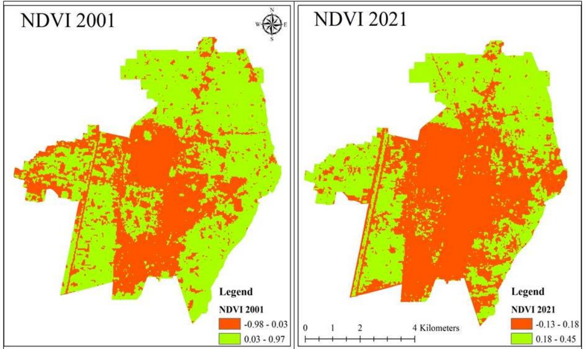
Figure 1. Normalized Difference Vegetation Index (2001 to 2021)
