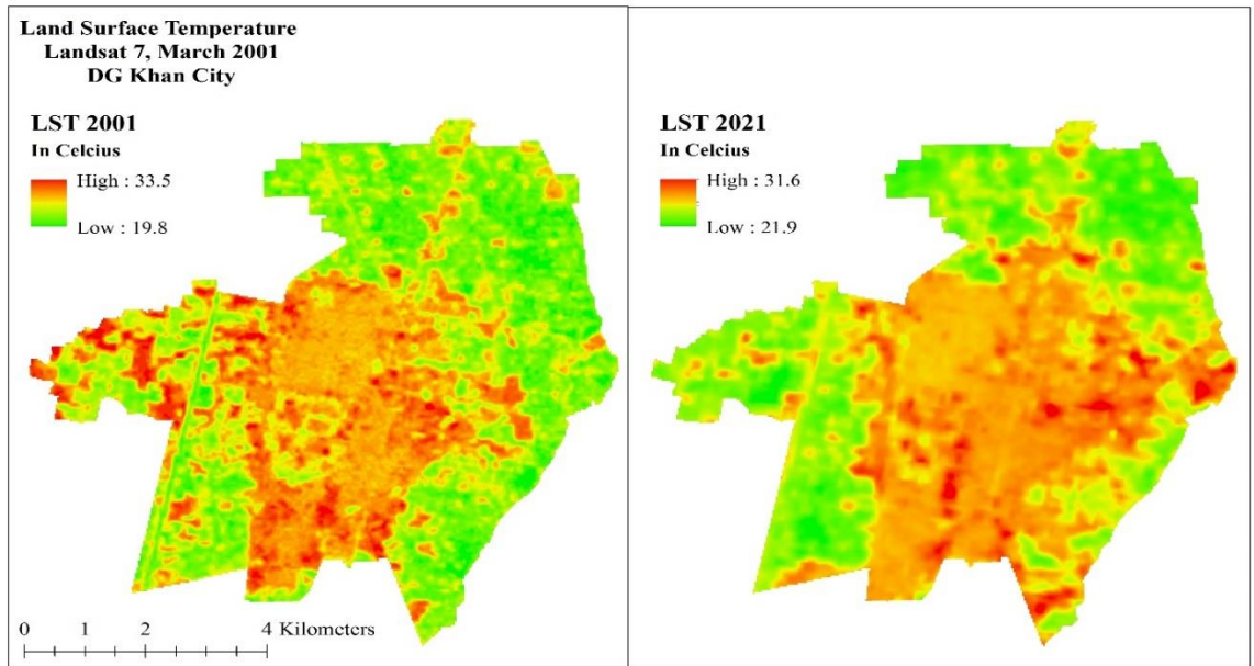
Figure 4. Land Surface Temperature (2001 to 2021)
