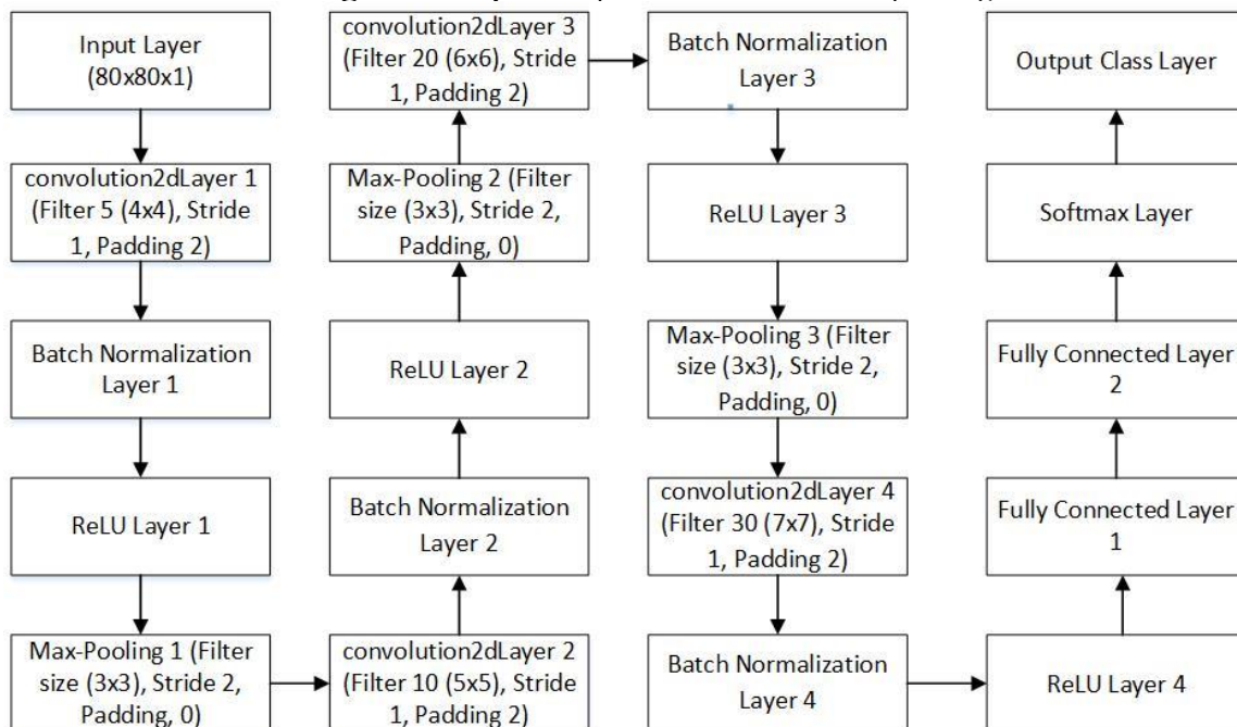
Figure 9. Basic architecture of 2D CNN.
