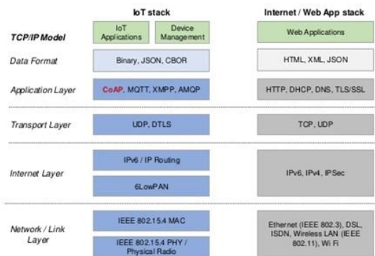
Fig. 2 Comparison between web and IoT protocol Stack
