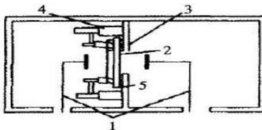
Figure 1. improved MIL-STD-285 test device
