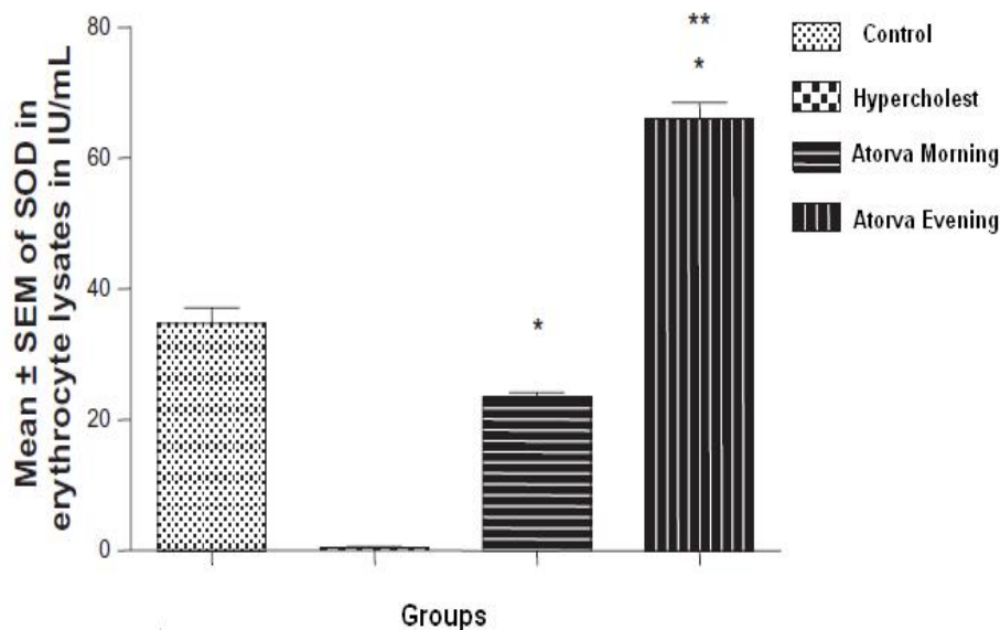
Figure 2: Effect of 8-weeks administration of Atorvastatin on superoxide dismutase [SOD] enzyme in IU/mL of erythrocyte lysates of the tested rabbits.
