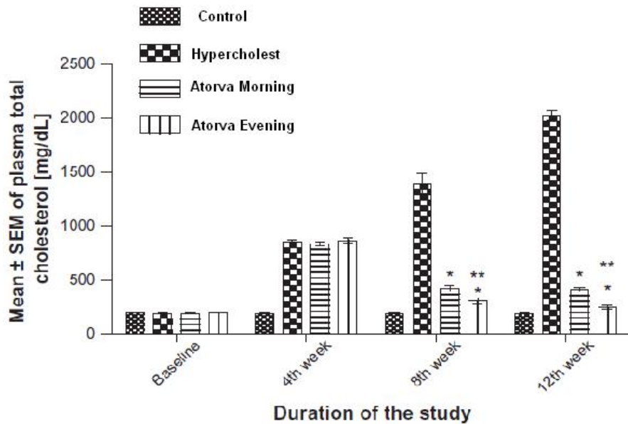
Figure 1: Effect of 8-weeks administration of Atorvastatin on plasma total cholesterol level in the tested rabbits.
