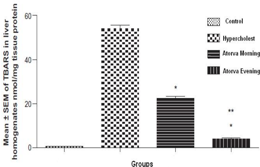
Figure 3: Effect of 8-weeks administration of Atorvastatin on thiobarbituric acid-reactive substance (TBARS) in nmol/mg tissue protein of the liver tissue homogenates of the Tested Rabbits.
