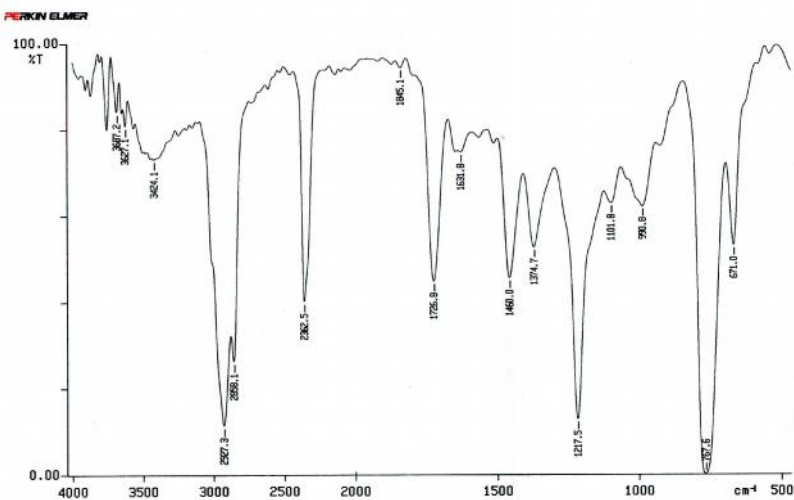
Figure 3: IR spectra of amentoflavone isolated from stem ethanolic extract of V.coriaceum
