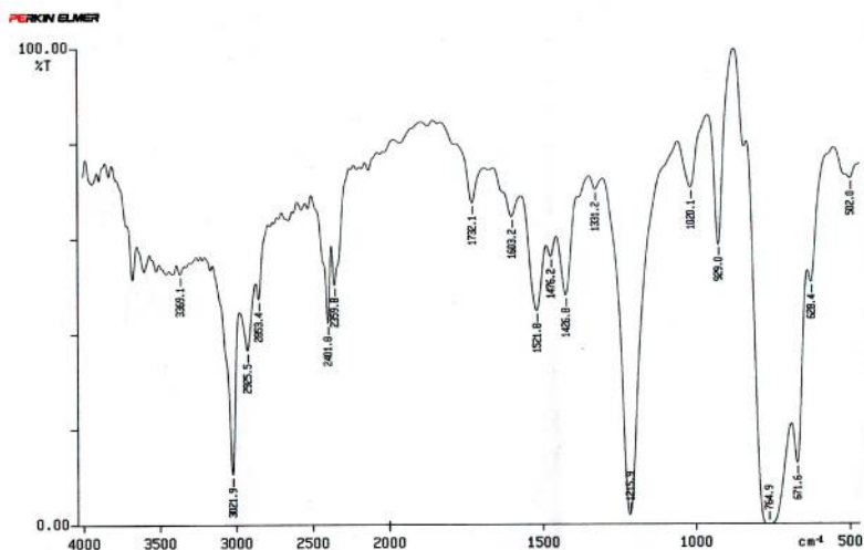
Figure 2: IR spectra of astragalgin isolated from stem ethanolic extract of V.punctatum
