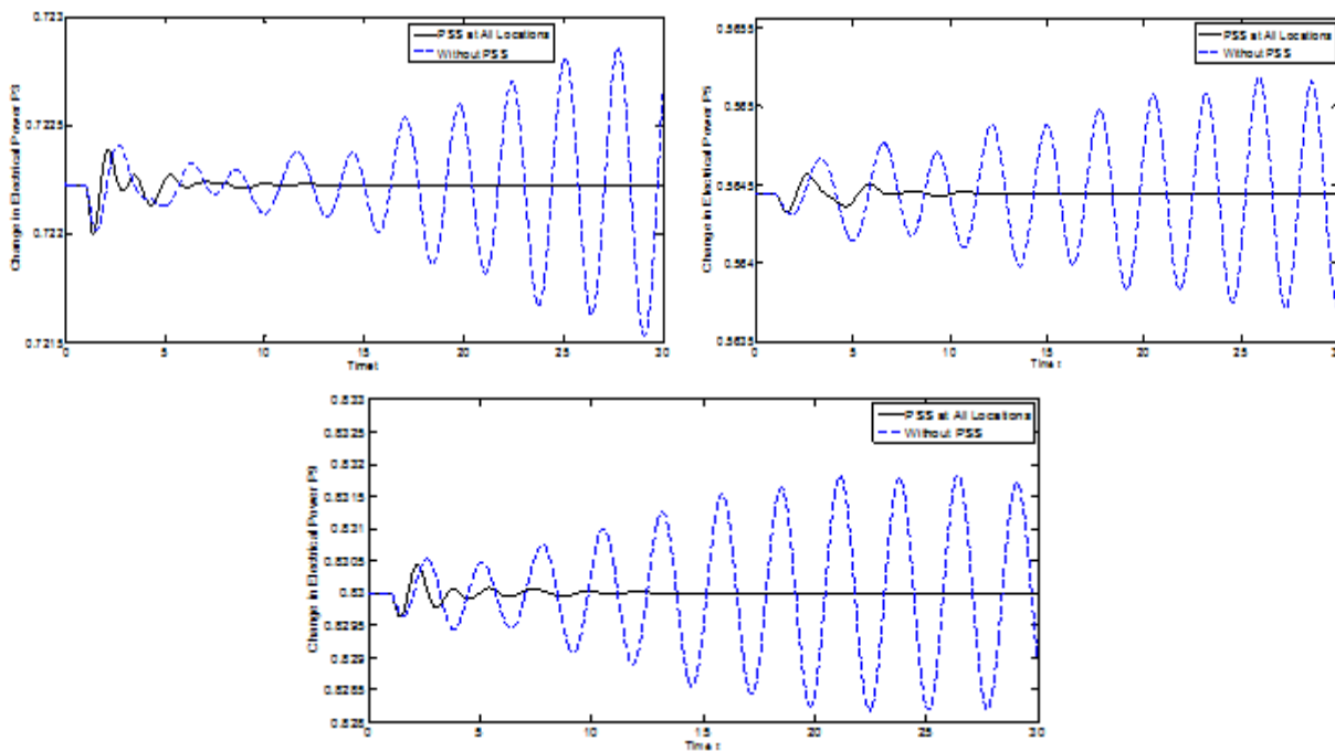
Figure 5 Change in Electrical power output of generators (a) G3, (b) G5 and (c) G9.
