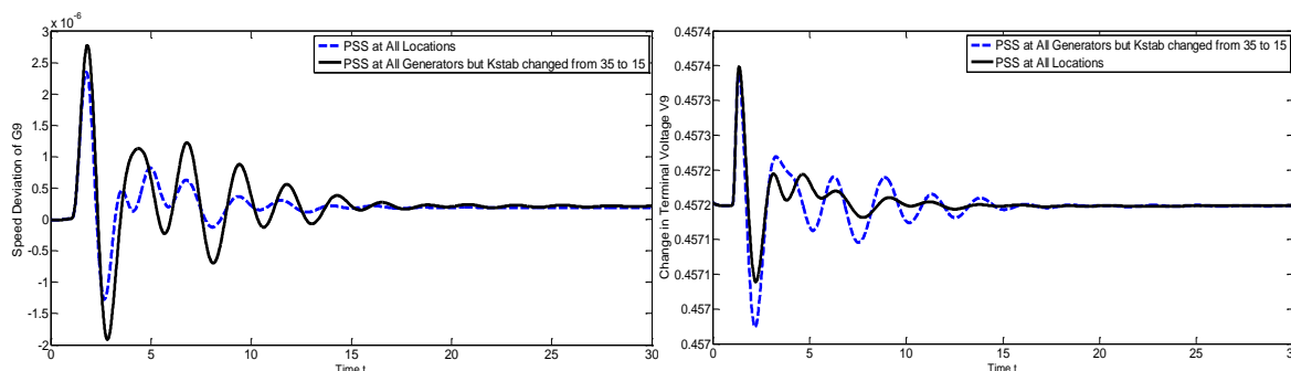
Figure 9 Speed deviation in Generator G9
