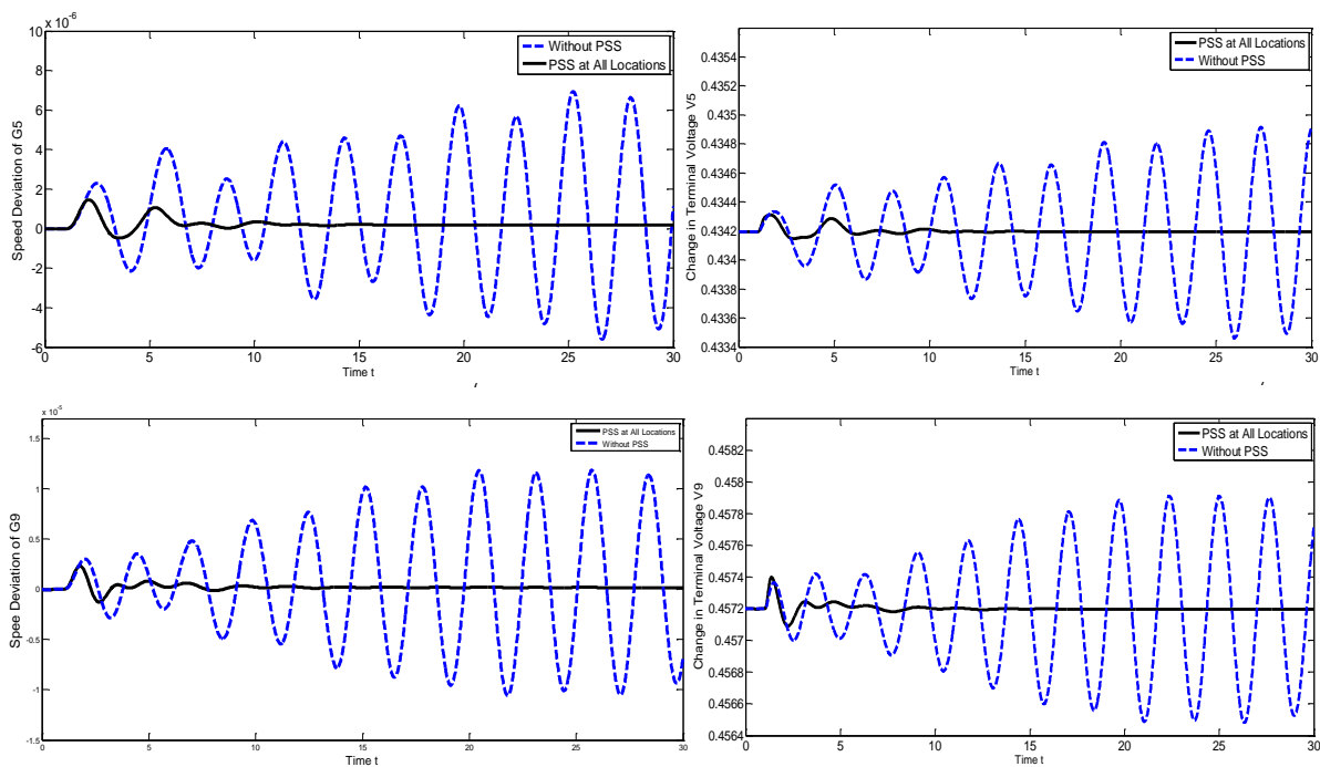
Figure 6 Speed deviation of (a) G3, (b) G5 and (c) G9 Figure 7 Change in Terminal Voltages of (a) G3, (b) G5 and (c) G9
