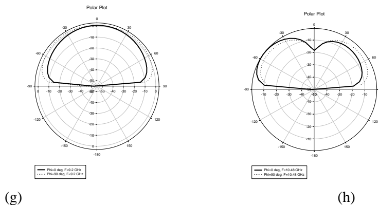
Figure. IV: Radiation patterns of the Antennas. (a) Antenna I at 5.2 GHz; (b) Antenna II at 8.3 GHz; (c) Antenna II at 9.7 GHz; (d) Antenna III at 8.2 GHz; (e) Antenna III at 9.8 GHz; (f) Antenna IV at 8.2 GHz; (g) Antenna IV at 9.2 GHz ; and (h) Antenna IV at 10.48 GHz
