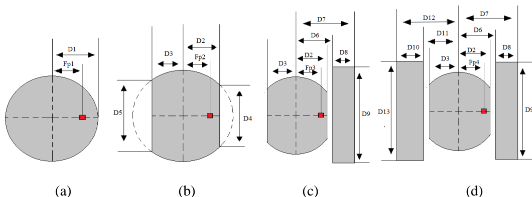
Figure. 1: Proposed Antenna Structure.
