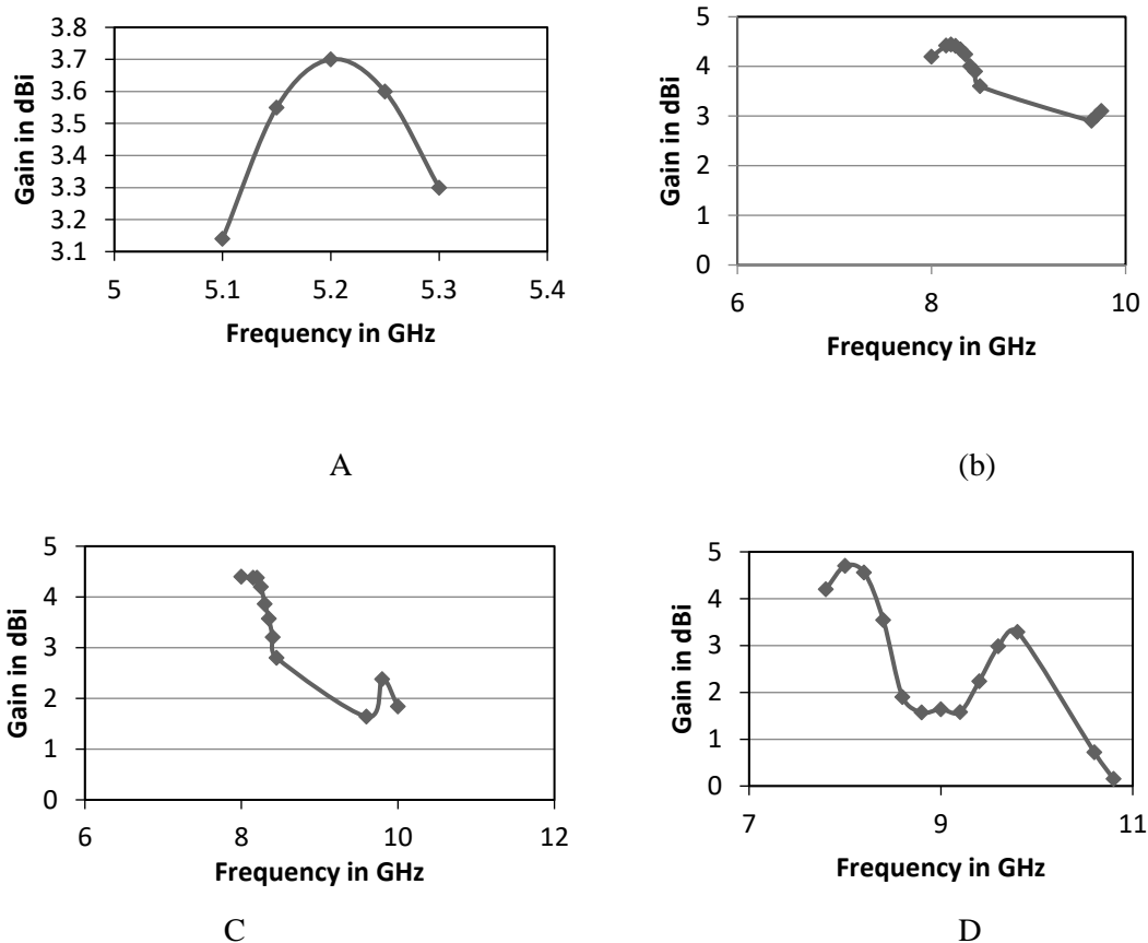
Figure. III: Frequency (GHz) versus Gain (dBi).
