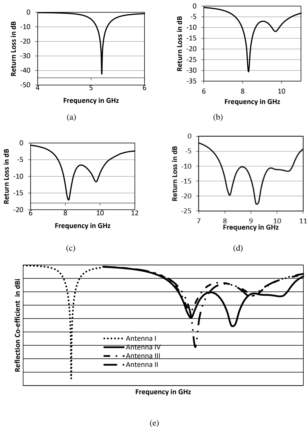
Figure. 2 Plot of frequency (GHz) versus return loss (dB).
