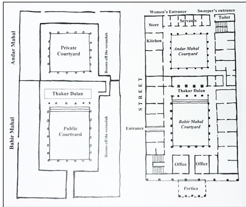
Figure 6 Generic plan and sample generated plan of indigenous house in old Kolkata
