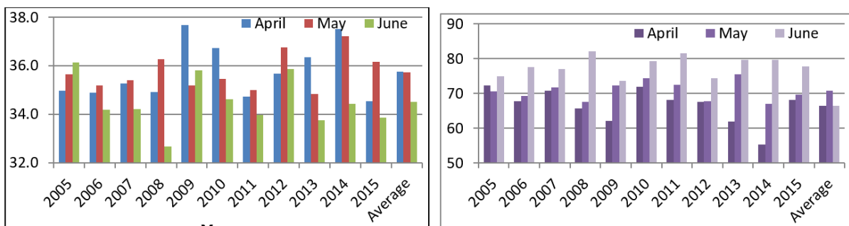
Figure 2 Average Maximum Outdoor Temperature and Relative Humidity of Kolkata during 2005-2015
