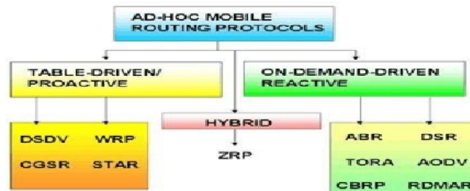
Figure 7 Adhoc routing protocols
