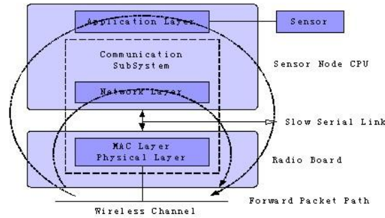
Figure 3 Architecture of sensor node
