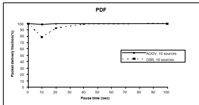
Figure 3 PDF for 10 Sources
