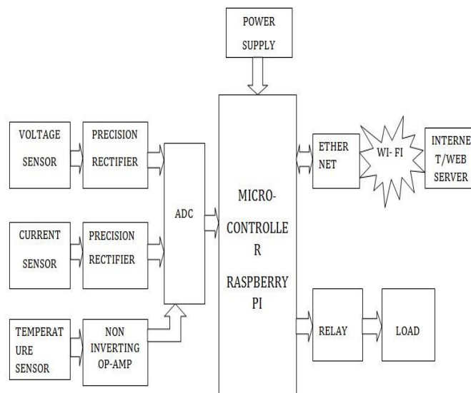
Figure 2 Client block diagram
