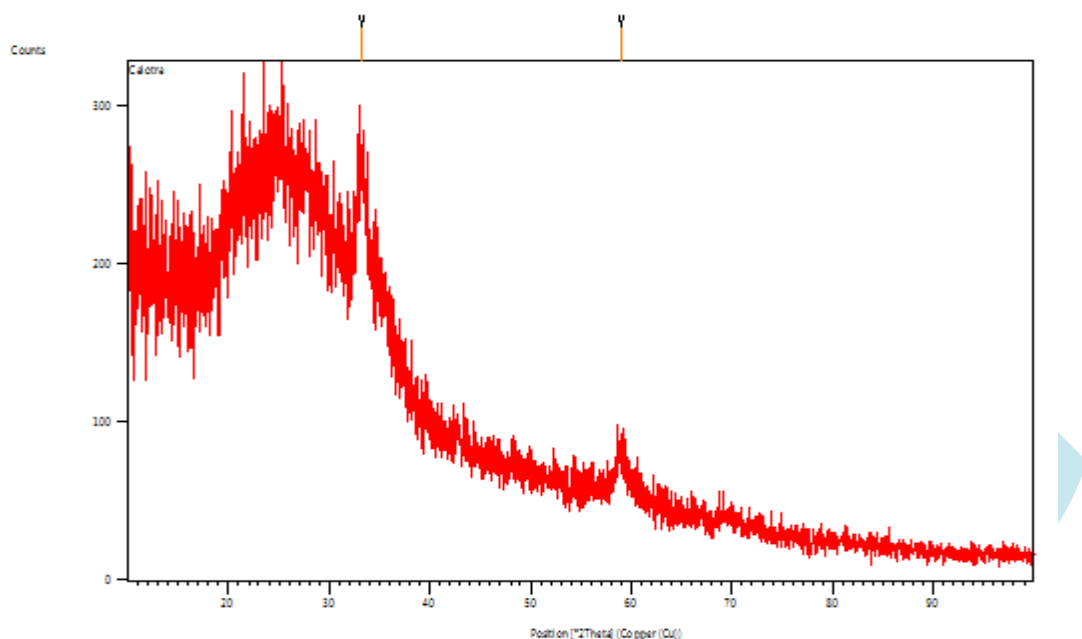
Fig. 4:- X-ray Diffraction Analysis (XRD)
