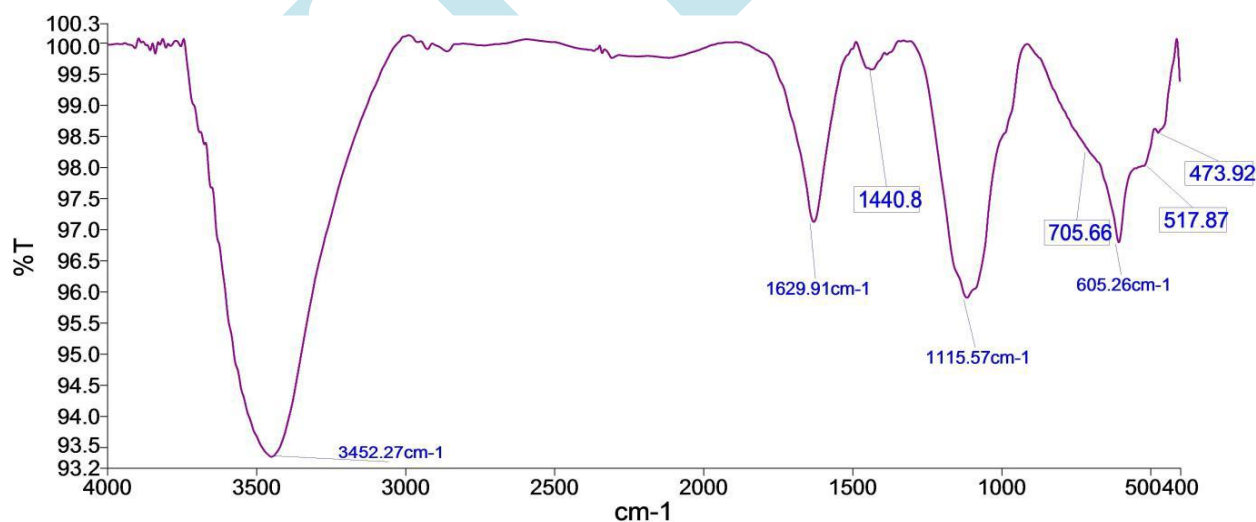
Fig. 3:- FTIR Analysis
