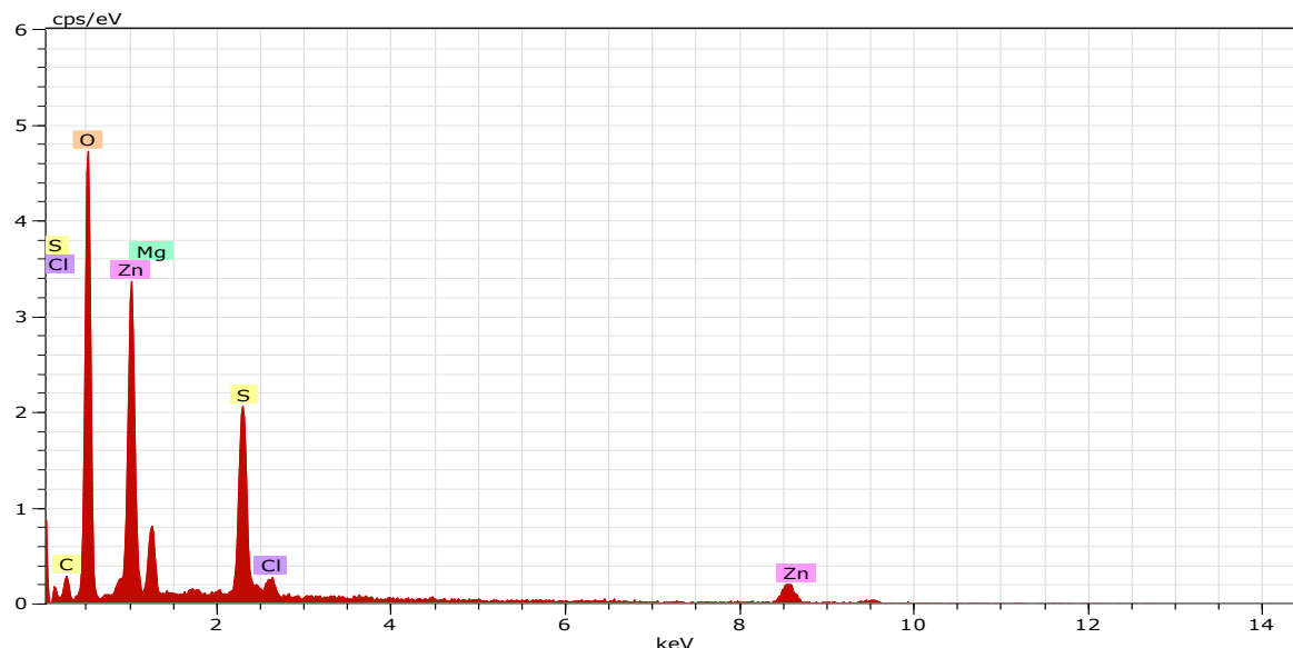
Fig. 5:- Energy Dispersive X-Ray Analysis (EDX)
