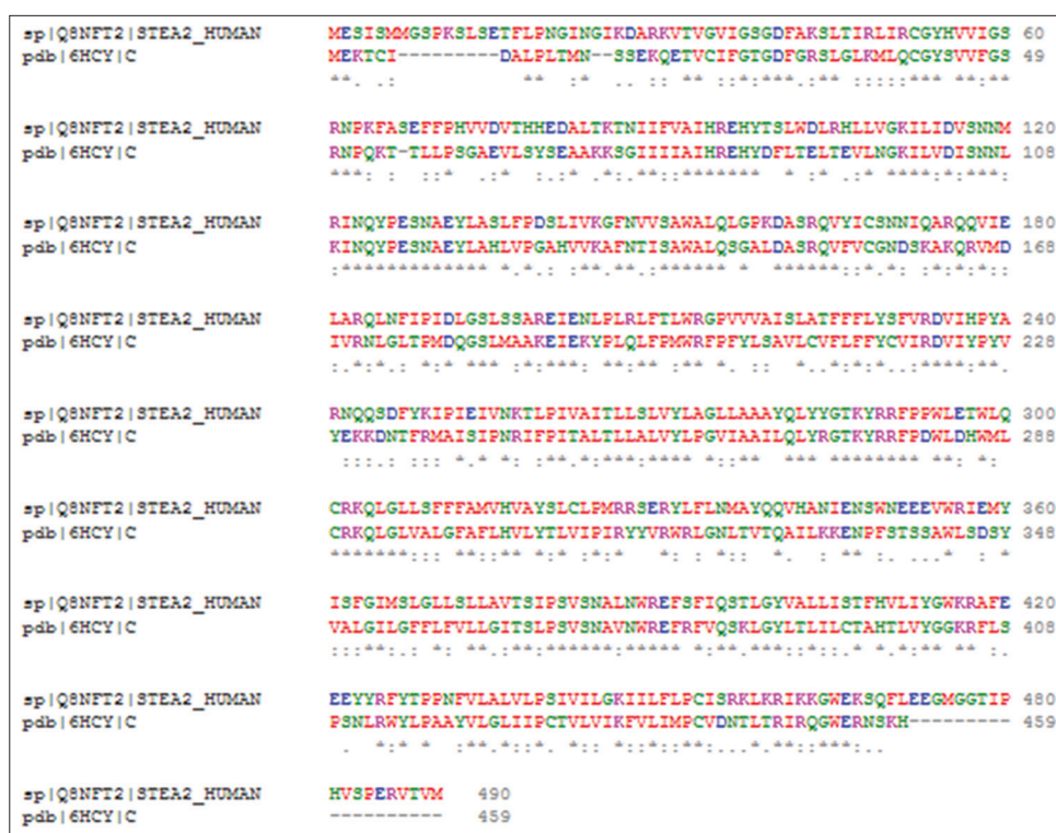
Figure 1: Sequence alignment of query sequence (metalloreductase STEAP2) and template sequence (6HCY)
