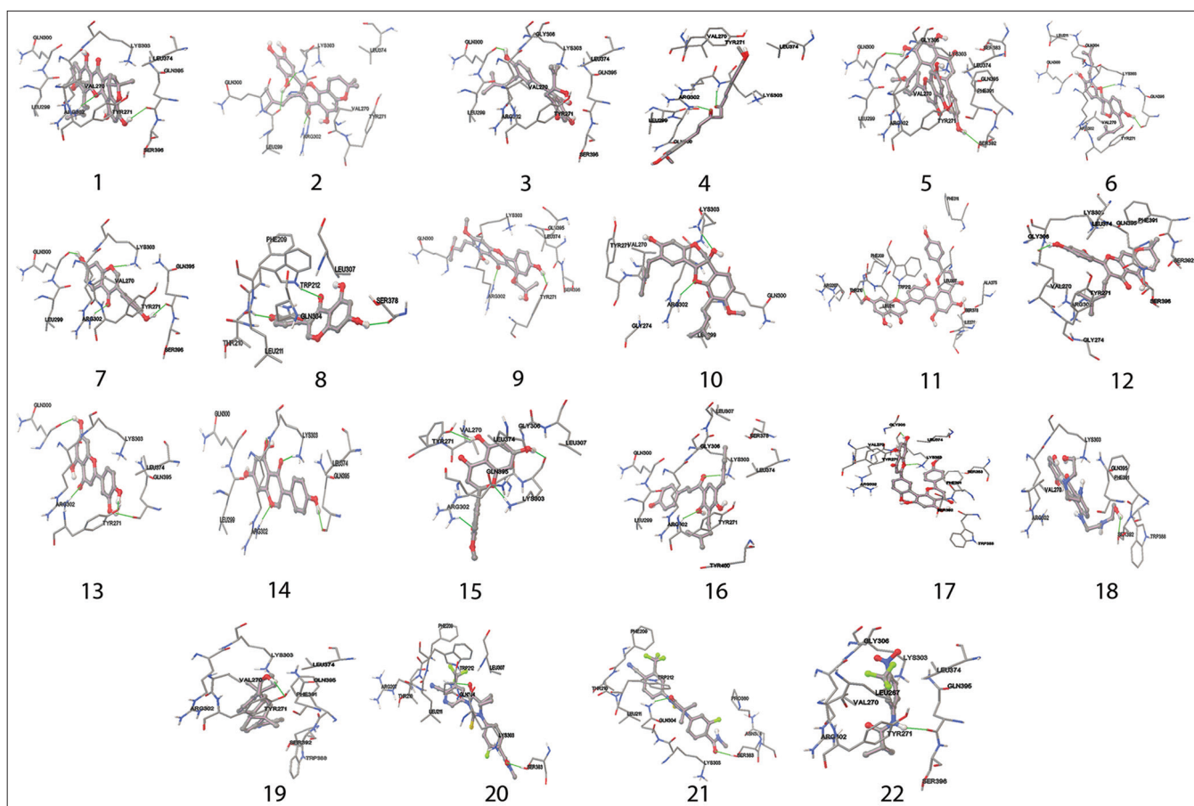
Figure 5: Docking of 17 natural compounds and standard drugs against modeled metalloreductase STEAP2 protein
