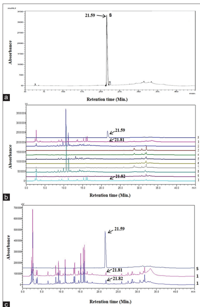
Figure 1: (a) High-performance liquid chromatography (HPLC) chromatogram of standard solasodine; (b) HPLC chromatogram of standard solasodine (S) with all the ten extracted samples (1-10), 1 – leaf methanol extract, 2 – bark hydro-alcohol extract, 3 – leaf n -hexane extract, 4 – leaf chloroform extract, 5 – bark ethyl acetate extract, 6 – bark n -hexane extract, 7 – leaf ethyl acetate extract, 8 – bark methanol extract, 9 – bark chloroform extract, and 10 – leaf hydro-alcohol extract; (c) A portion enlarged HPLC chromatogram of standard solasodine (S) with standard samples 1 and 10
