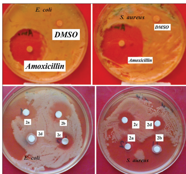
Figure 9: Antibacterial activity of nitrones against Escherichia coli and Staphylococcus aureus bacteria
