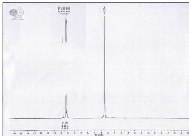
Figure 7: 1 H-Nuclear magnetic resonance spectrum of 2c
