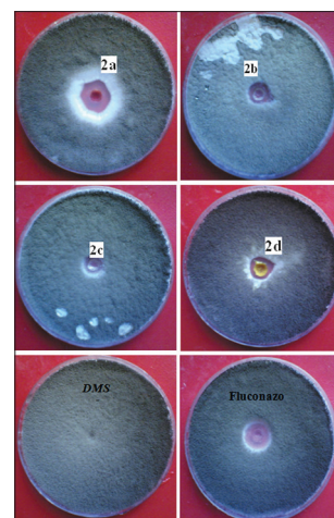
Figure 10: Antifungal activity of nitrones against Aspergillus niger fungi
