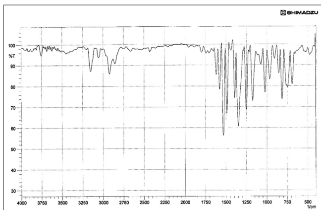
Figure 2: Fourier transform infrared spectrum of nitrono compound 2b
