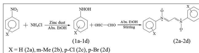
Scheme 1: Synthetic routes of nitron compounds
