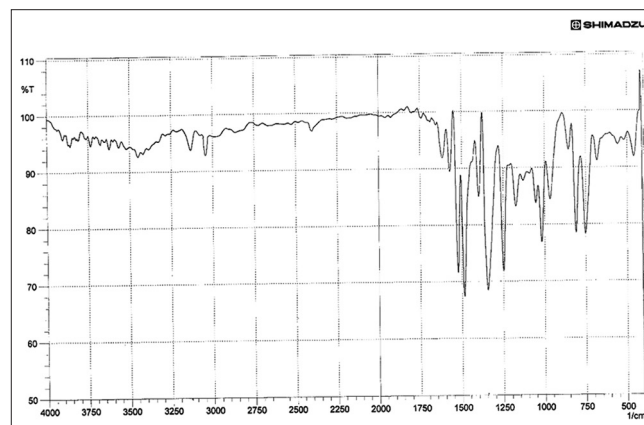
Figure 3: Fourier transform infrared spectrum of nitrono compound 2c
