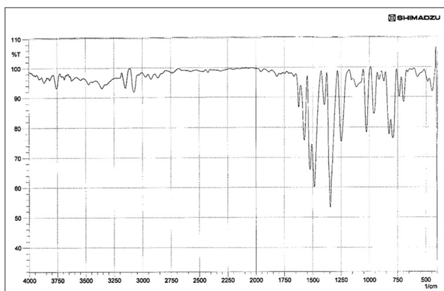
Figure 1: Fourier transform infrared spectrum of nitrono compound 2a
