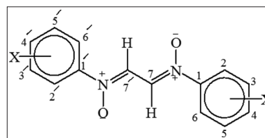
Scheme 2: Structure of synthesized nitrones for explanation 1 H-NMR
