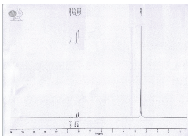
Figure 8: 1 H-Nuclear magnetic resonance spectrum of 2d
