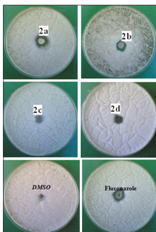
Figure 11: Antifungal activity of nitrones against Aspergillus flavus fungi
