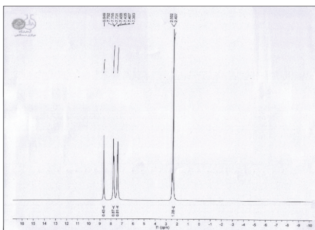
Figure 6: 1 H-Nuclear magnetic resonance spectrum of 2b
