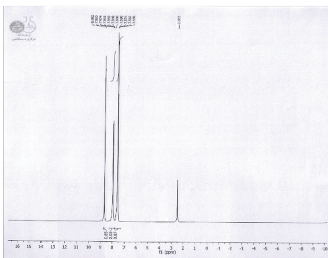
Figure 5: 1 H-Nuclear magnetic resonance spectrum of 2a
