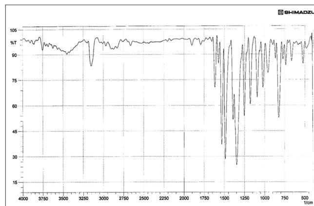
Figure 4: Fourier transform infrared spectrum of nitrono compound 2d
