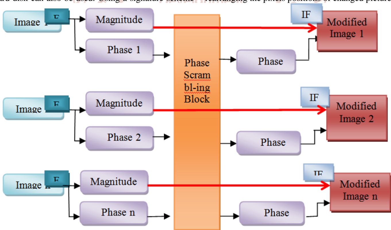
Fig. 2 Block Level Structure of Multiple Multimedia data (Image) encryption
