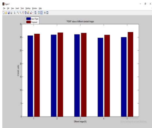
Fig. 7 Graphical comparison of PSNR
