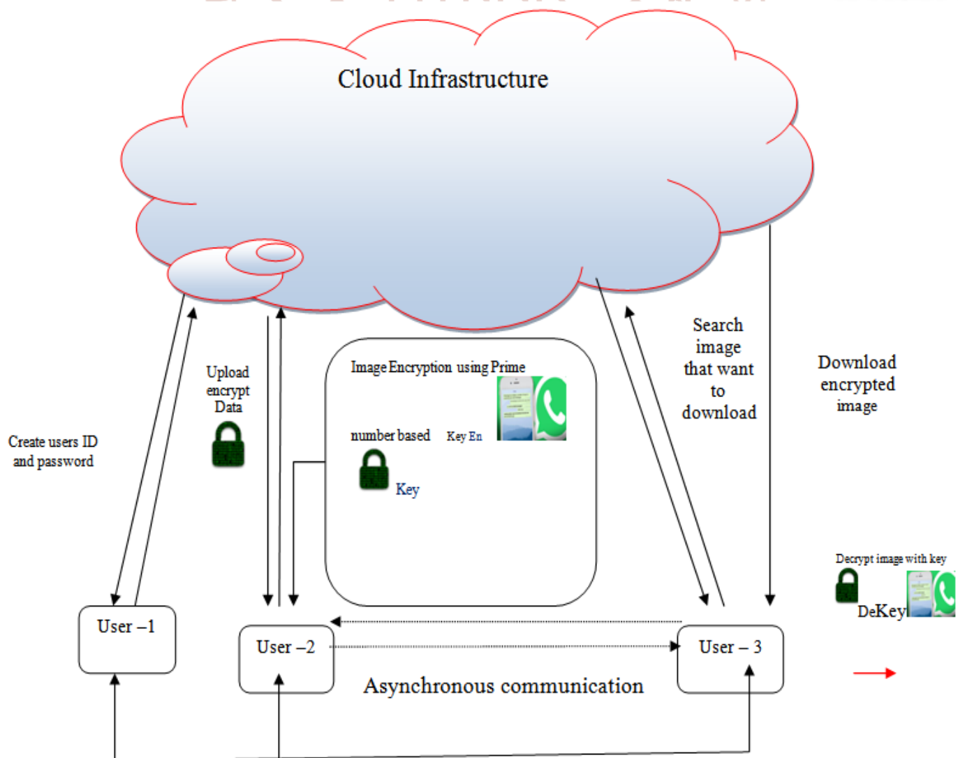
Fig. 3 Block diagram of Proposed Method
