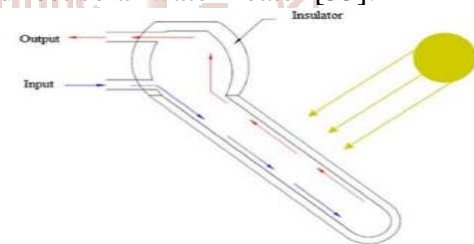
Fig.7. Schematic Direct Solar Water Heater
