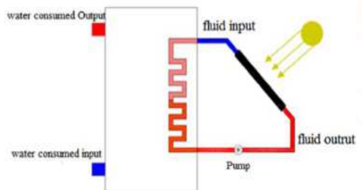
Fig.8. Schematic Indirect Solar Water Heaters
