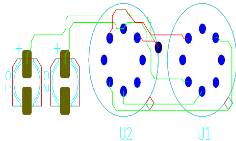
Fig.2(d): ultiboard design of HPF circuit
