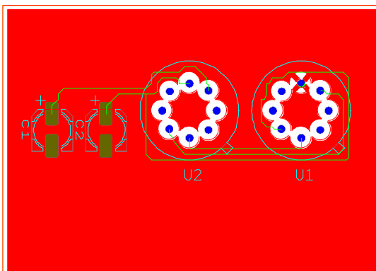
Fig.2(e):PCB layout using Ultiboard of HPF
