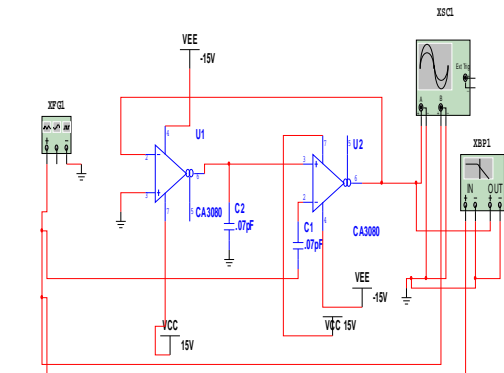
Fig 2. :HPF circuit
