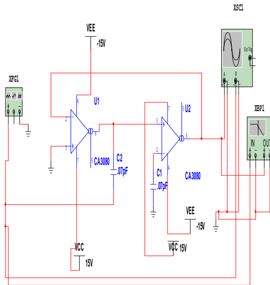
Fig.3 : BPF circuit
