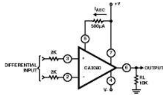
Fig(ii) schematic diagram of CA3080IC
