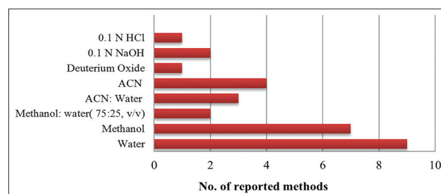
Figure 2: Various diluents used for the analysis of citicoline
