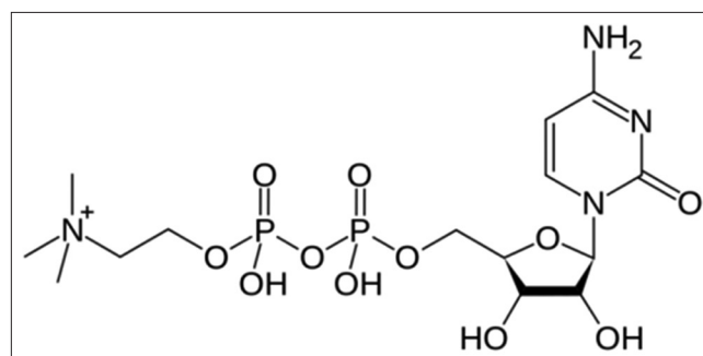
Figure 1: Structure of citicoline
