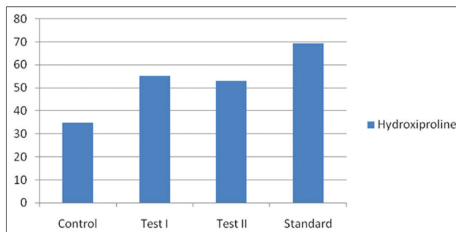
Graph 5: Effect of extract on hydroxiproline estimation
