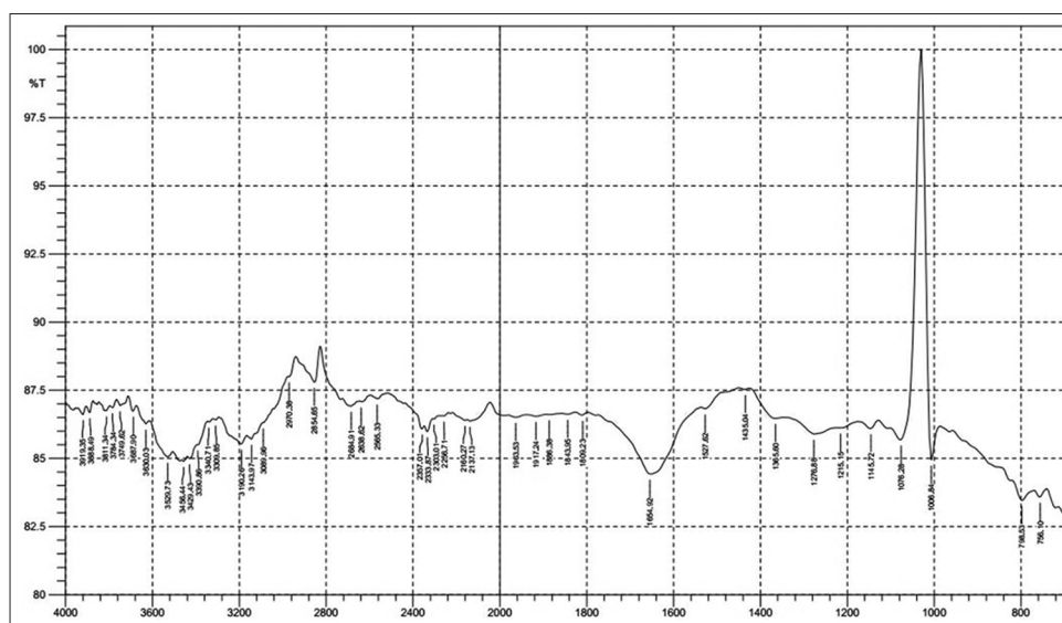
Figure 2: Fourier transform-infrared spectrum analysis in methanolic leaf extract of Dodonaea viscosa
