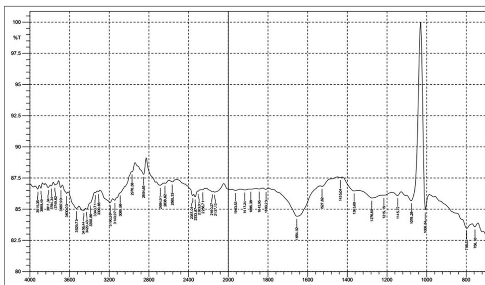
Figure 1: Fourier transform-infrared spectrum analysis in petroleum ether leaf extract of Dodonaea viscosa
