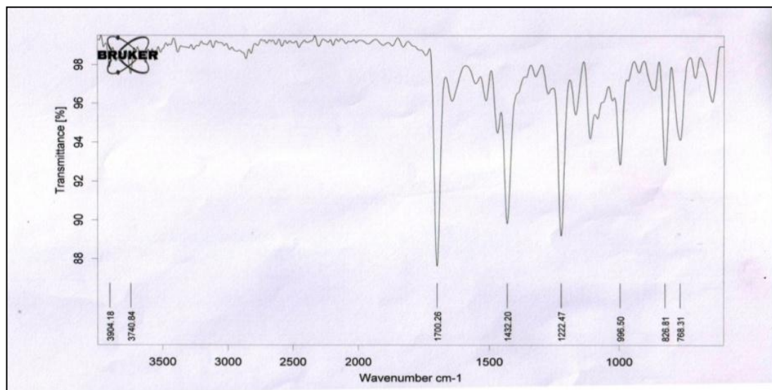
Fig.2: FTIR spectrum of Loratadine Sample
