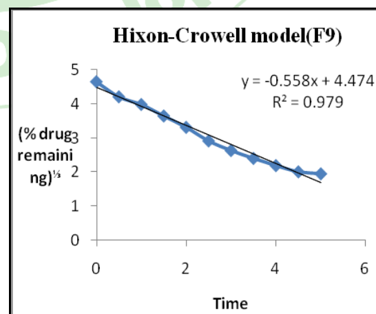
Fig.16: Hixon-Crowell plot for F9
